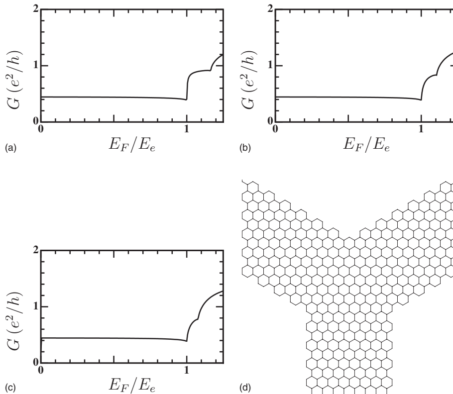
FIG. 7. Conductance per spin of triangles with three armchair nanoribbon leads having N transverse channels, with ribbons connecting to the triangle along their narrower cross section. (a) N=5 , (b) N=8 , (c) N=11 , (d) Geometry for N=8 .
