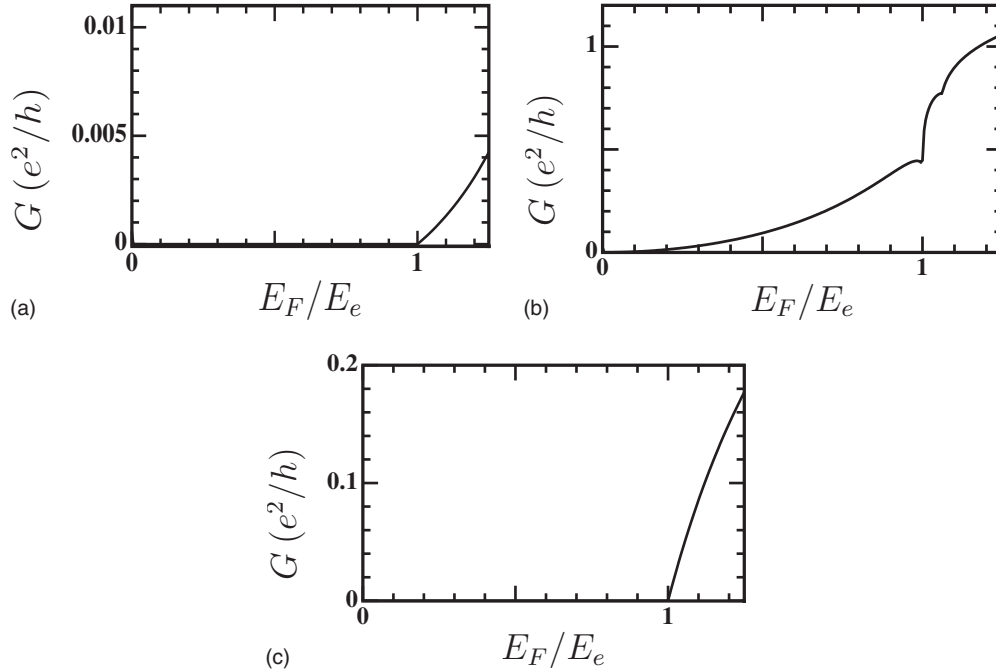
FIG. 15. Conductance per spin in the low-energy region for an equilateral triangle with three armchair leads. (a) N=13 , (b) N=14 , (c) N=15 .
