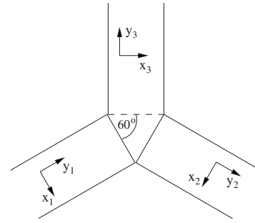
FIG. 3. Schematic diagram of an equilateral triangle with three armchair leads, in which the triangle is taken as an “end cap” for the vertical lead. Coordinates for the three sections illustrated. Wave functions must be matched along the two solid lines of the triangle.
