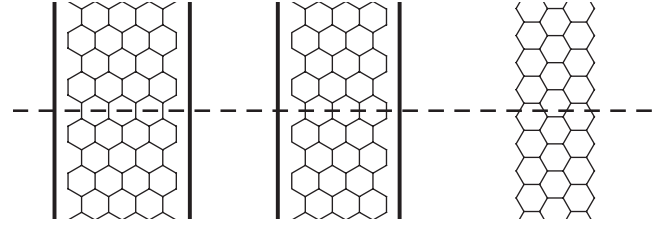
FIG. 13. Symmetric armchair, asymmetric armchair, and zigzag ribbons with N=4 . The dashed line cuts through four bonds of each ribbon, the minimal number required to sever each into two disconnected pieces. Heavy vertical lines indicate rows of fictive lattice points along which the wave function vanishes for the armchair nanoribbons.
