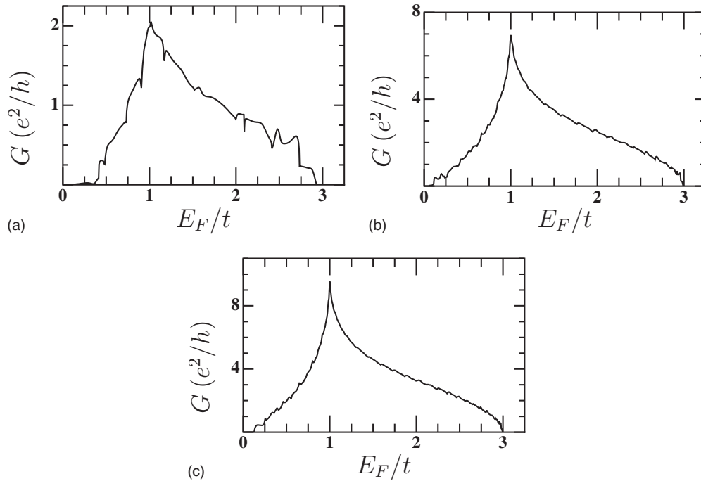
FIG. 17. Conductance per spin for two leads at an angle of 120^\circ , through a hexagon with six armchair leads. (a) N=5 , (b) N=15 , (c) N=20 .
