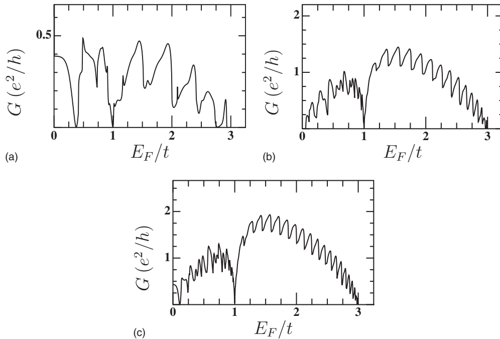
FIG. 16. Conductance per spin for two leads at an angle of 60^\circ , through a hexagon with six armchair leads. (a) N=5 , (b) N=15 , (c) N=20 .
