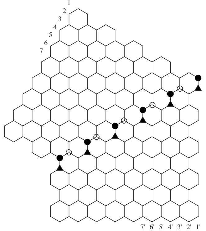
FIG. 8. Diagram detailing the joining surface between leads for the simple 120^\circ bend, as well as the labeling scheme for x and x' coordinates. Matching the wave function on the dark circles and triangles accounts for current continuity across the joining surface.
