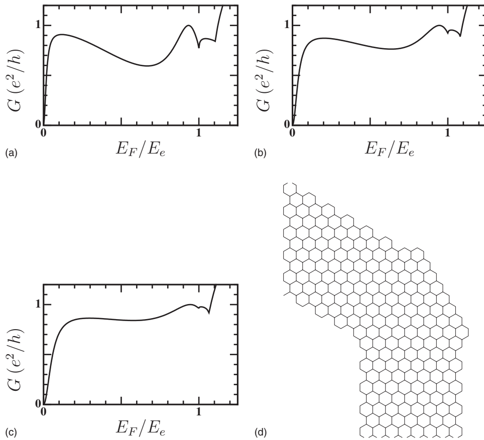
FIG. 5. Conductance per spin of triangles with two armchair nanoribbon leads having N transverse channels. (a) N=5 , (b) N=11 , (c) N=14 , (d) Geometry for N=8 .
