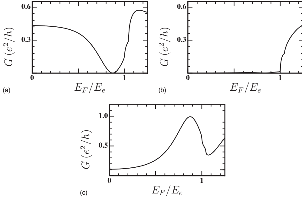
FIG. 19. Conductance per spin for two leads at an angle of (a) 60^\circ , (b) 120^\circ , and (c) 180^\circ through a hexagon with six N=20 armchair leads.
