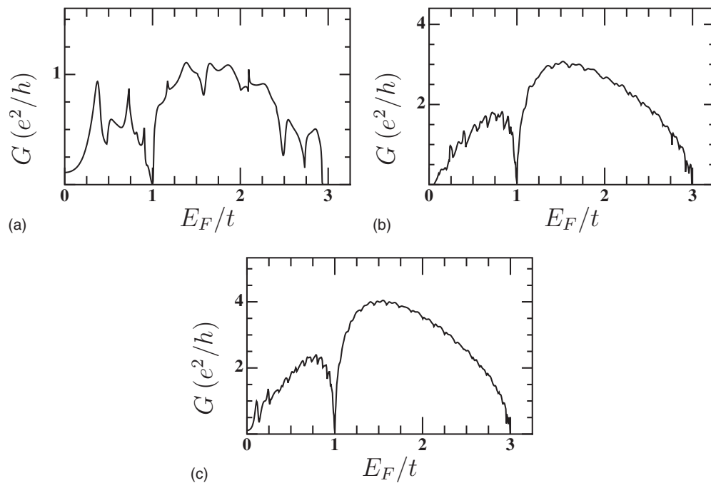
FIG. 18. Conductance per spin for two leads at an angle of 180^\circ , through a hexagon with six armchair leads. (a) N=5 , (b) N=15 , (c) N=20 .
