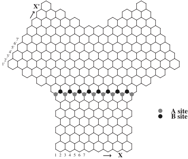
FIG. 9. Diagram detailing the joining surface between the lower lead and the upper left lead, for an equilateral triangle with three leads, and the leads attached to the triangle at the wider point in their cross section.
