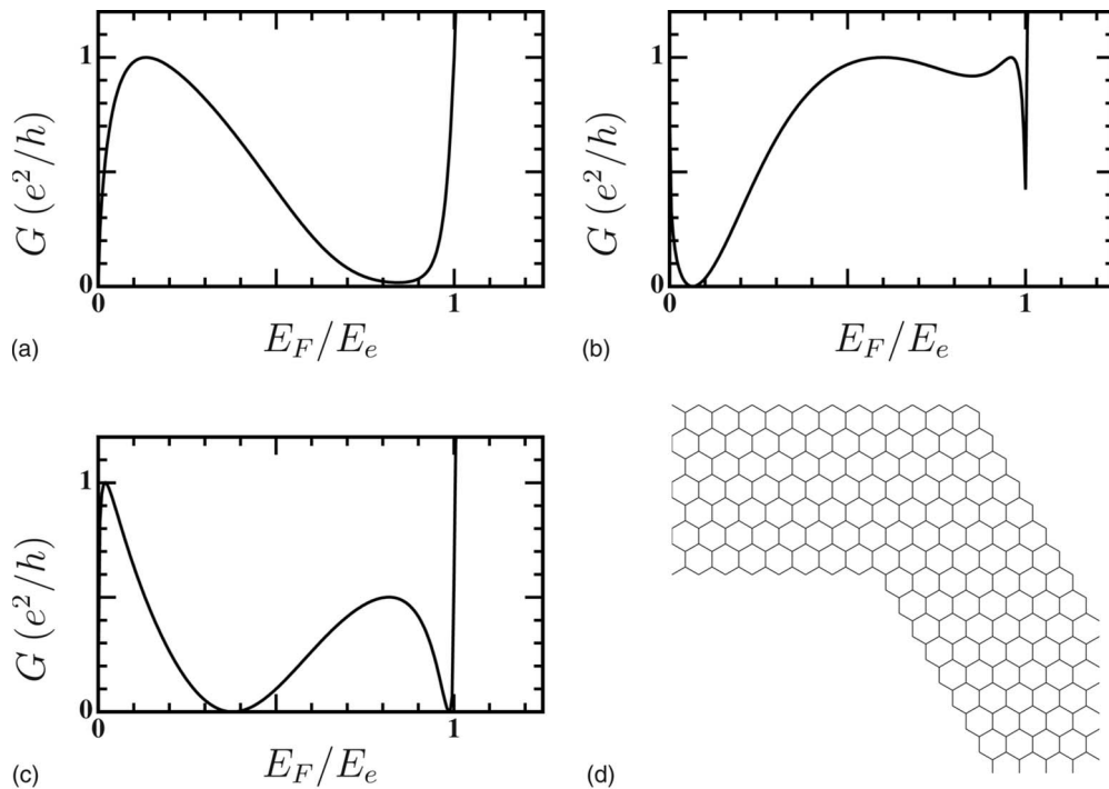
FIG. 20. Transmission through 120^\circ bend for zigzag ribbons. (a) N=6 , (b) N=7 , (c) N=8 . (d) Geometry for N=8 .
