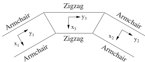
FIG. 2. Schematic diagram of a 120^\circ armchair junction, in which electrons pass through a length of zigzag ribbon. Coordinates for the three sections illustrated. Wave functions must be matched along the two solid lines connecting the armchair ribbons to the zigzag ribbon.
