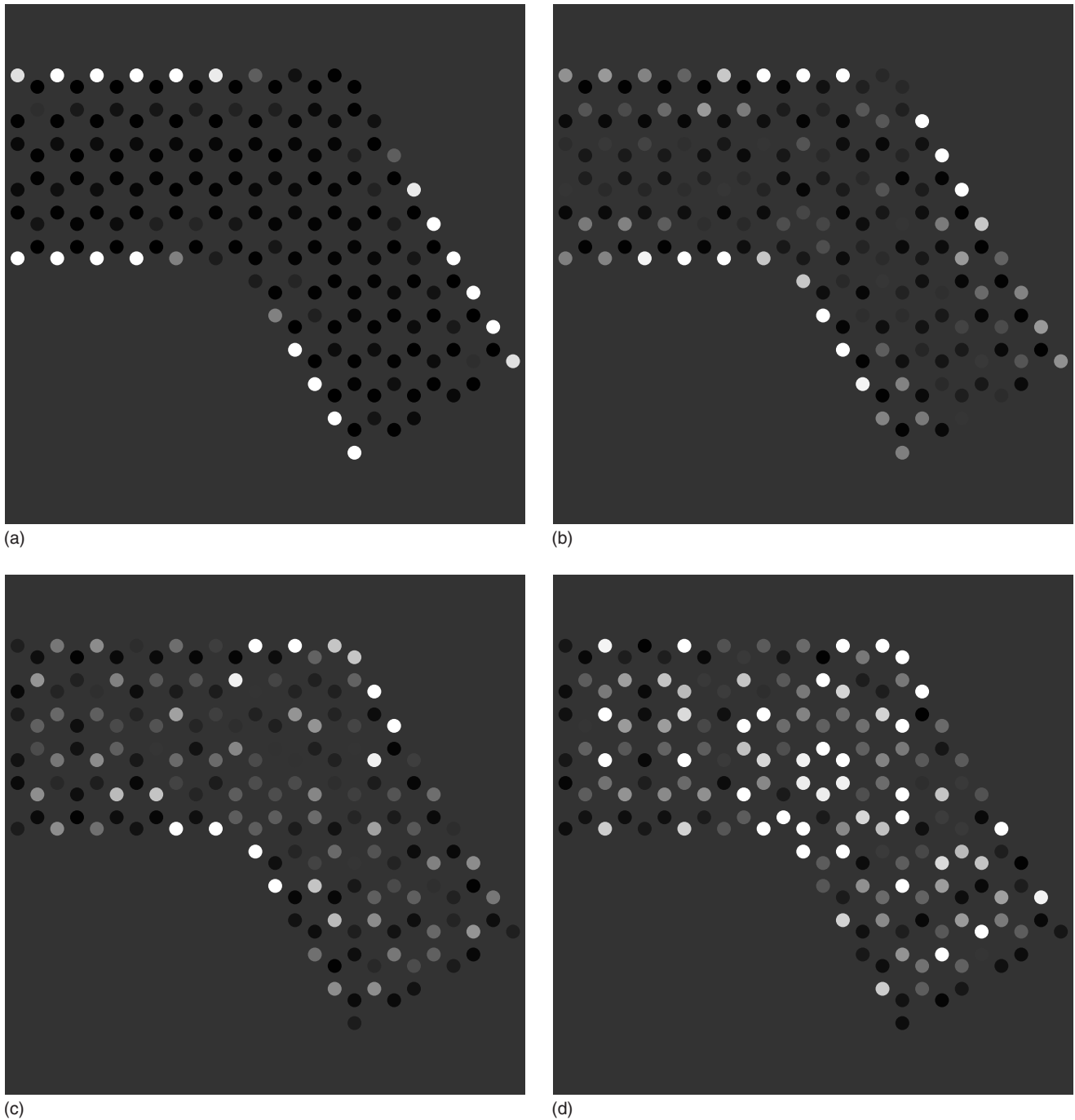
FIG. 21. Local density of states (LDOS) shown in grayscale for 120^\circ zigzag junction, N=6 . Black denotes zero, and white denotes maximal LDOS. The leads modeled in the calculation extend away from the junction to infinity. (a) E_F/E_E=0.016 , (b) E_F/E_E=0.016 , (c) E_F/E_E=0.49 , (d) E_F/E_E=0.82 .
