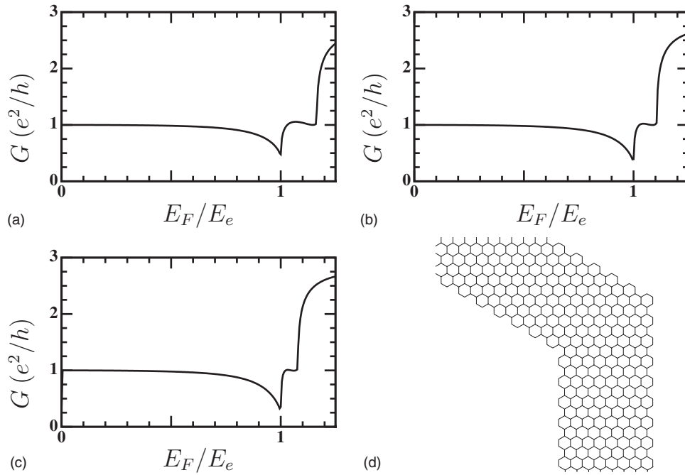
FIG. 4. Conductance per spin of 120^\circ bends in armchair nanoribbons having N transverse channels. (a) N=5 , (b) N=8 , (c) N=11 , (d) Geometry for N=8 .
