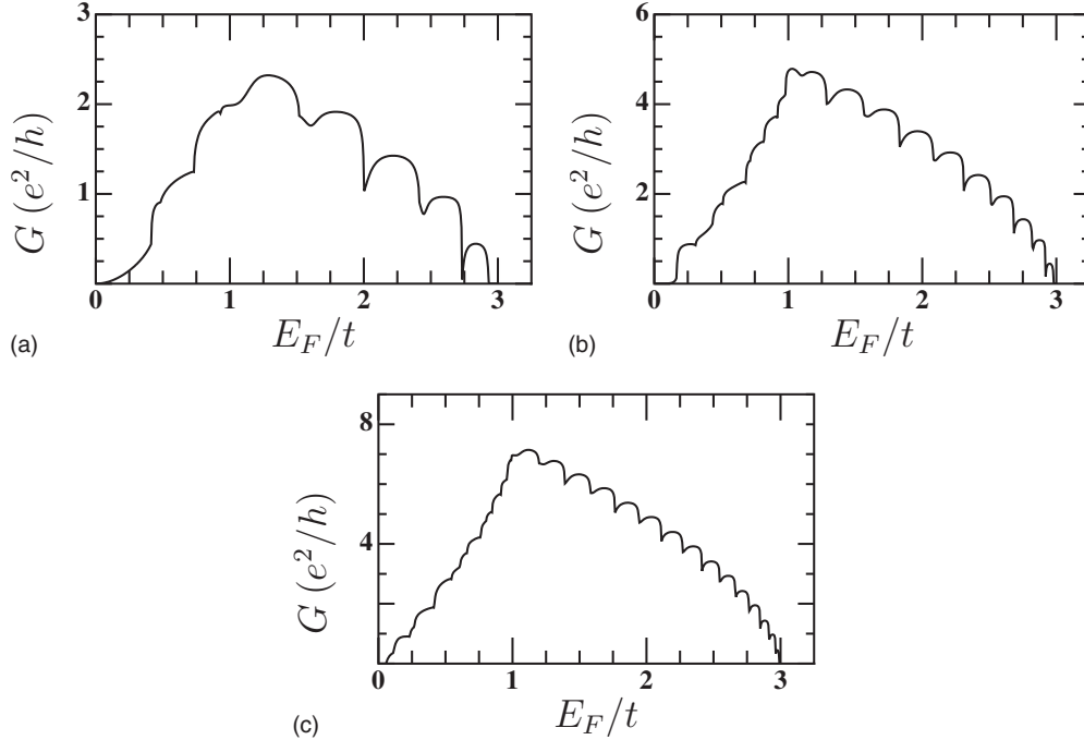
FIG. 14. Conductance per spin through an equilateral triangle with three armchair leads of sizes (a) N=5 , (b) N=10 , and (c) N=15 .
