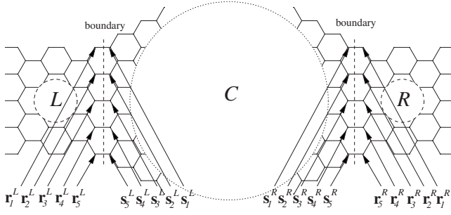
FIG. 12. Conceptual division of the geometry into regions C , L , and R , illustrating the lattice point labeling scheme at the boundaries, which are denoted by vertical dashed lines. This example has symmetric armchair ribbons with N=4 , and the boundary is chosen such that Q=5 .
