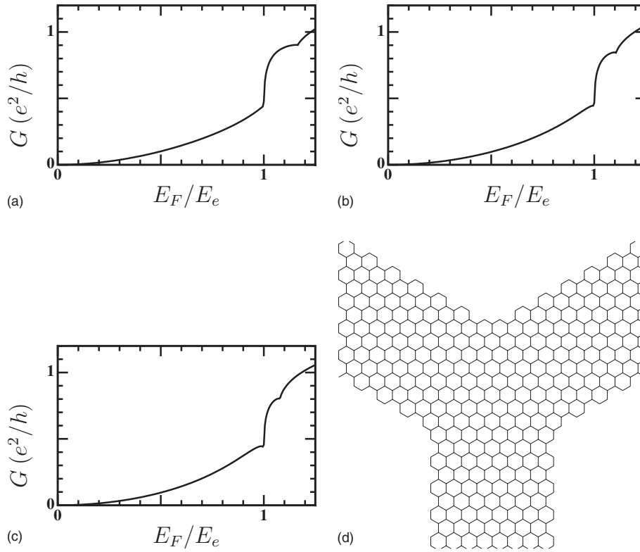
FIG. 6. Conductance per spin of triangles with three armchair nanoribbon leads having N transverse channels, with ribbons connecting to the triangle along their wider cross section. (a) N=5 , (b) N=8 , (c) N=11 , (d) Geometry for N=8 .
